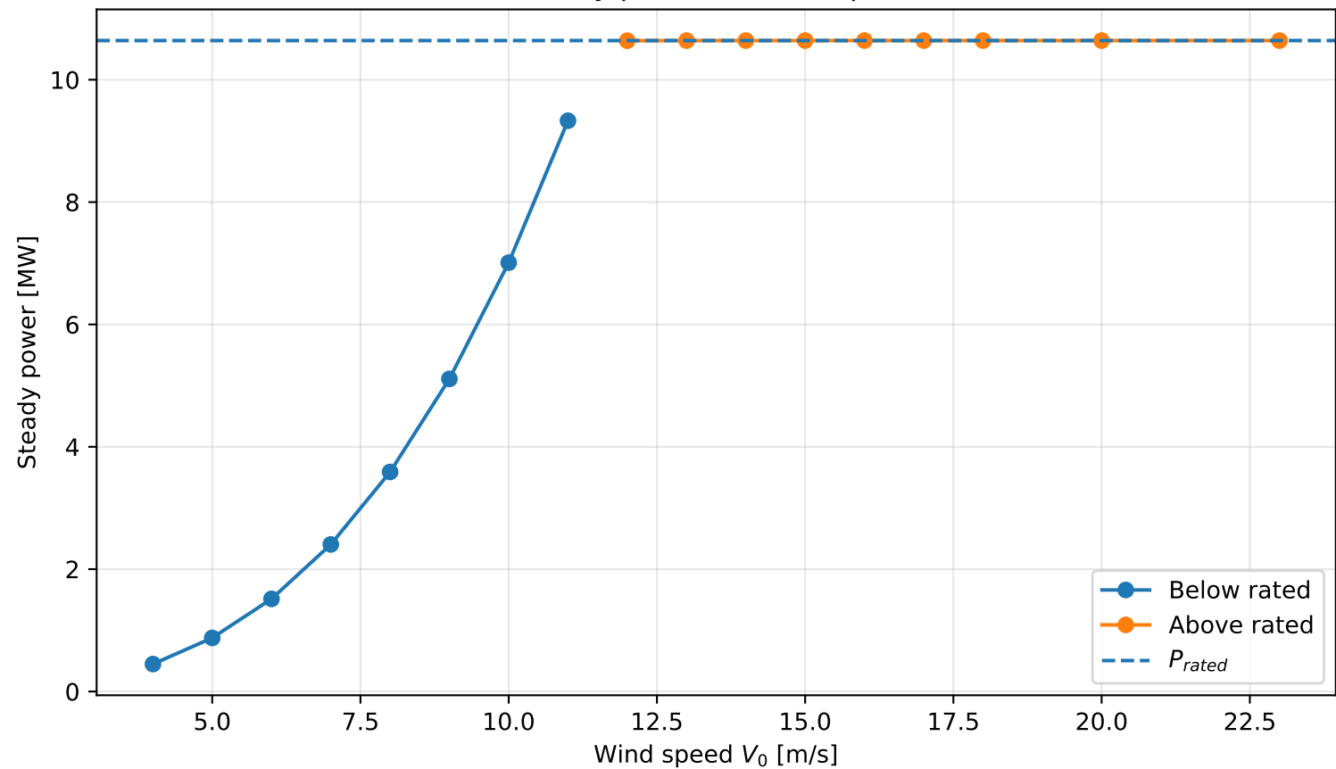
Steady power vs wind speed
